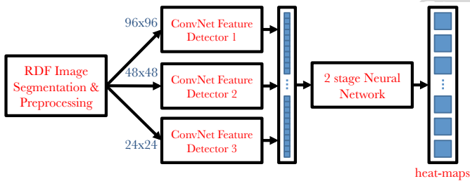
Fig. 6: Convolutional Network Architecture
