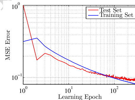
Fig. 13: ConvNet Learning Curve
