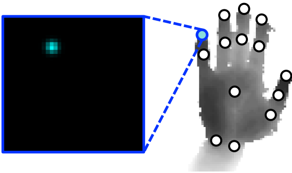
Fig. 5: Depth image overlaid with 14 feature locations and the heat-map for one fingertip feature.
