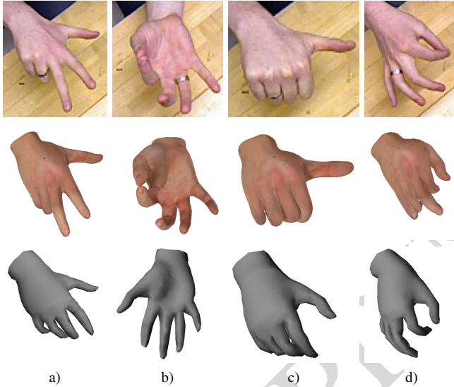
Fig. 17: Comparison with state-of-the-art commercial system: RGB ground-truth (top row), this work inferred model [Šarić 2011] pose (middle row), [3Gear 2014] inferred model pose (bottom row) (images used with permission from 3Gear).
