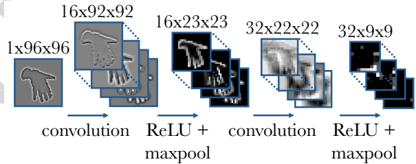
Fig. 8: High-Resolution Bank Feature Detector: each stage: ( N_{\text{features}} \times \text{height} \times \text{width} )
