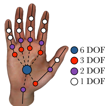
Fig. 3: Linear Blend Skinning (LBS) Model [Šarić 2011] with 42 DOF
