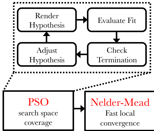
Fig. 4: Algorithm Pipeline For Dataset Creation
