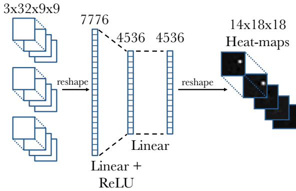
Fig. 9: 2-Stage Neural Network To Create The 14 Heat Maps (with sizing of each stage shown)
